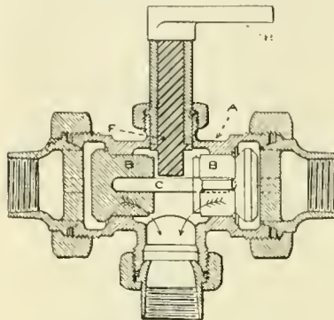
DETAILS OF CYLINDER COCK.
